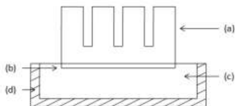
Figure 1: solid fin with heater and heat sink
