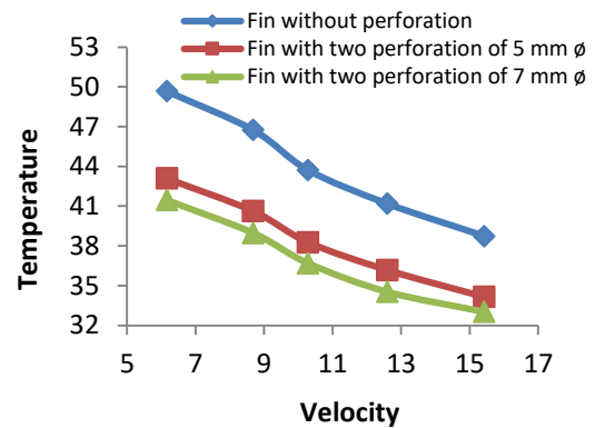
Fig. 8: Effect of Velocity on temperature of fin
