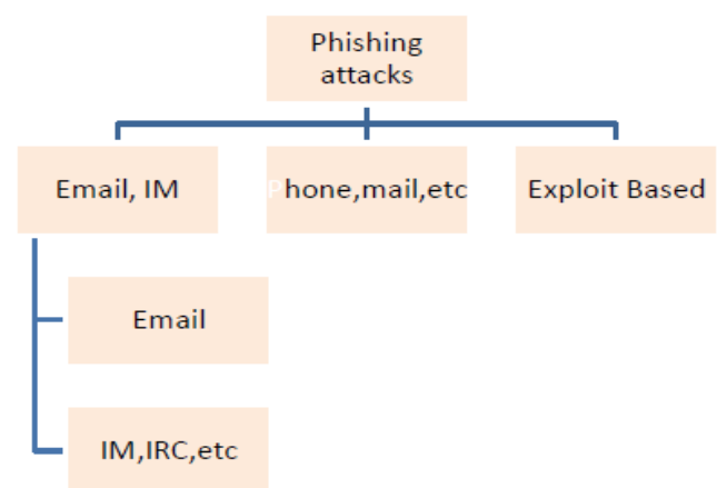
Fig1. Phishing Attacks
