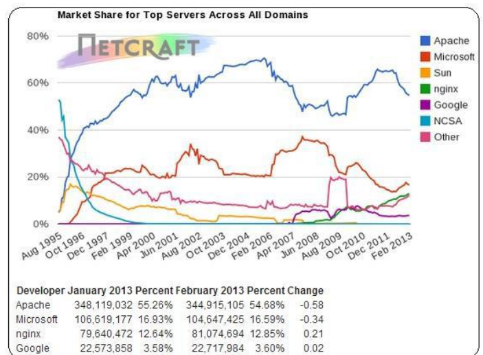
Fig5. Netcraft's survey
