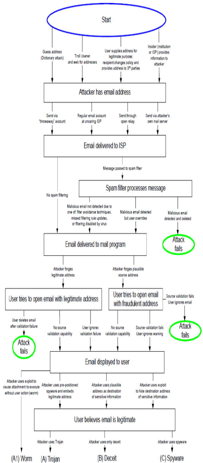
Fig3. Stages in phishing attack
