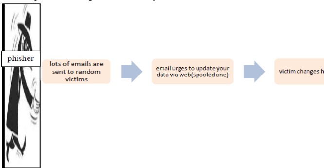
Fig2. Phishing Process
