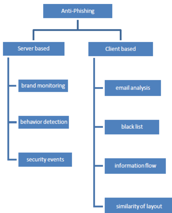
Fig4. Anti-phishing techniques
