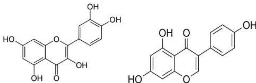
Figure 16. Molecular mechanisms of flavonoids on melanin synthesis [167]. Mushroom tyrosinase has been widely used as a substitute for mammalian tyrosinase to screen for tyrosinase inhibitors as it is inexpensive and commercially available in a purified form. Soy isoflavones are attractive source of functional cosmetic materials with anti-wrinkle, whitening and skin hydration effects. For quercetin, two studies showed stimulatory effect and one showed an inhibitory effect for melanogenesis. Genistein also exhibited melanogenic effect. So, the skin whitening of soya bean may be explained by some other mechanism(s).
