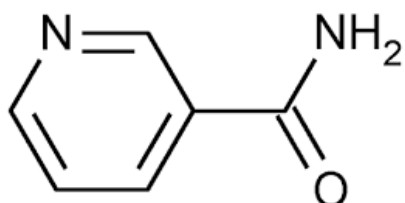
Figure 15. Niacinamide
