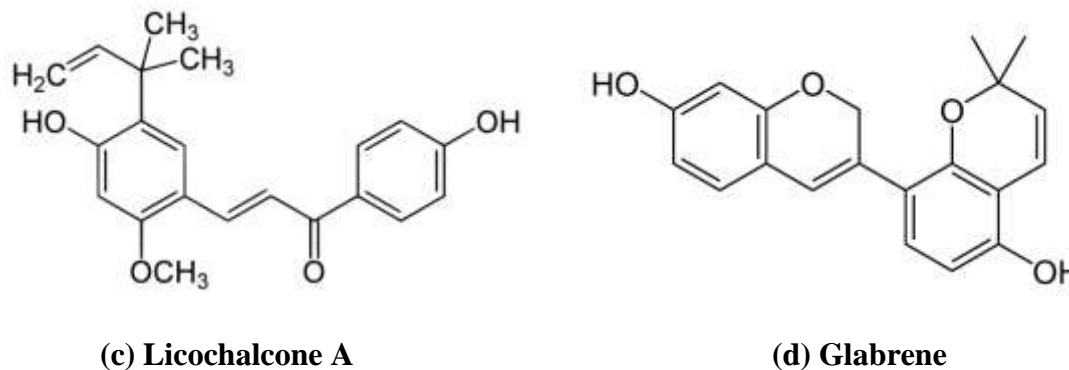
Figure 11. Important Licorice ingredients for skin depigmenting, lightening
