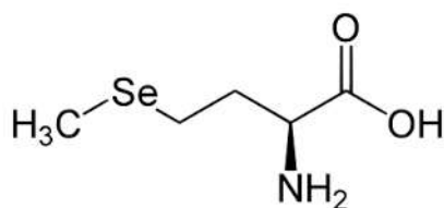
(b) L-selenomethionine
