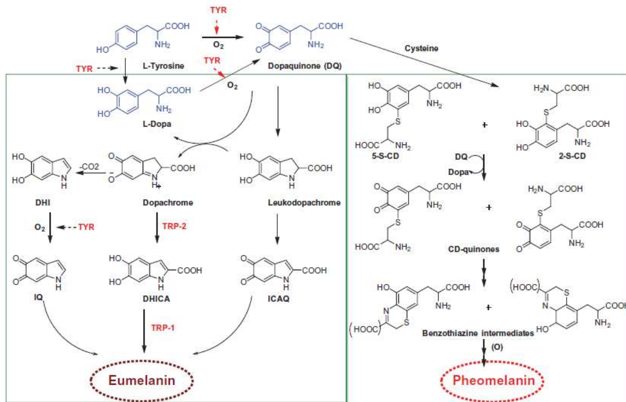
Figure 3. Melanogenesis pathway (production of eumelanin and pheomelanin) [1]. (Tyr: tyrosinase; DQ: dopaquinone; L-Dopa: L-3:4-dihydroxyphenylalanine; DHICA: 5,6-dihydroxyindole-2 carboxylic acid; DHI: 5,6-dihydroxyindole; ICAQ: indole-2-carboxylic acid-5,6-quinone; IQ: indole-5,6-quinone; HBTA: 5-hydroxy-1,4-benzothiazinylalanine).
