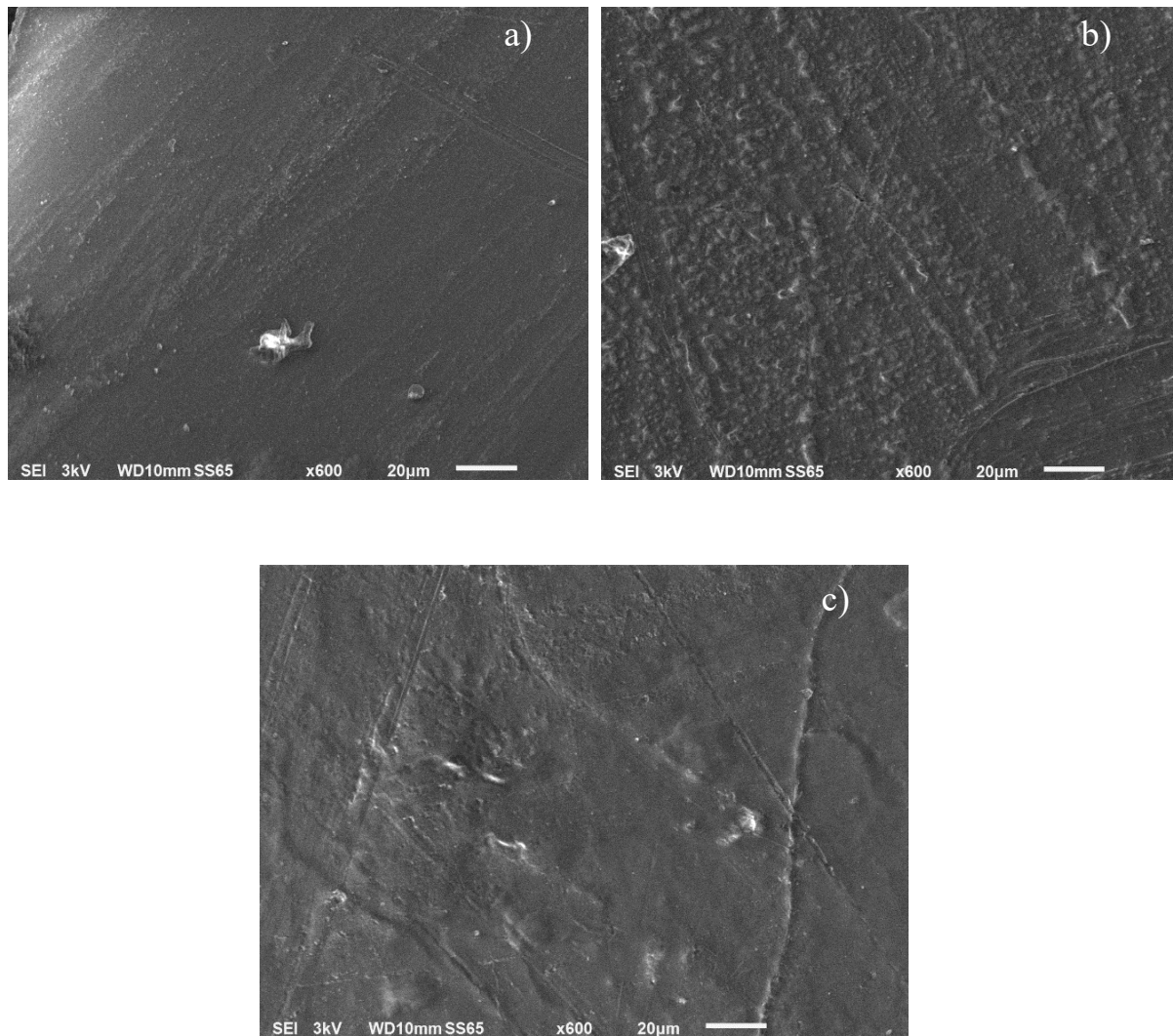
Figure 3. SEM micrographs of starch-based bioplastic: (a) control, (b) A 1 and (c) A 2 .
